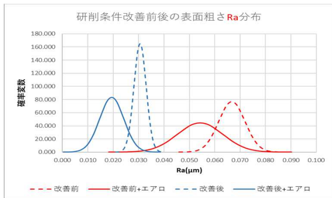
SKD11 (1辺40mm)
